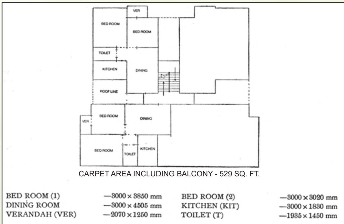
FLOOR PLAN
